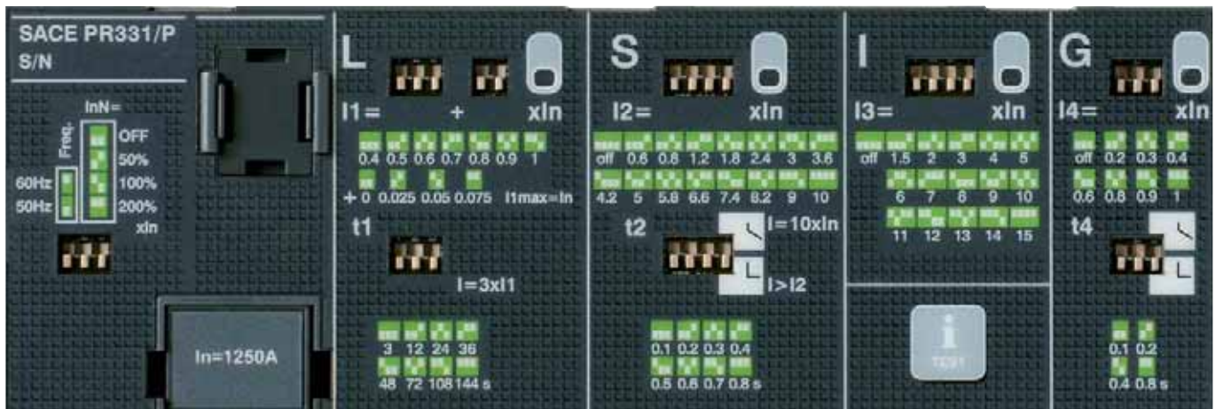
PR331/P LSIG
